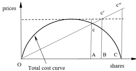
Figure 1: Schema between profits and shares in light of the profit line and total cost curve.
